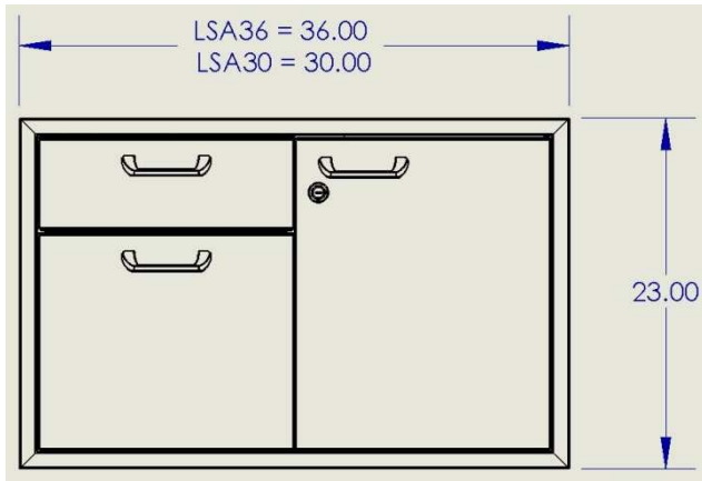
Overall Dimensions
